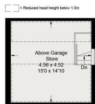
Garage - First Floor
